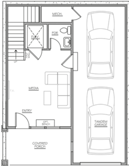
LOWER LEVEL
