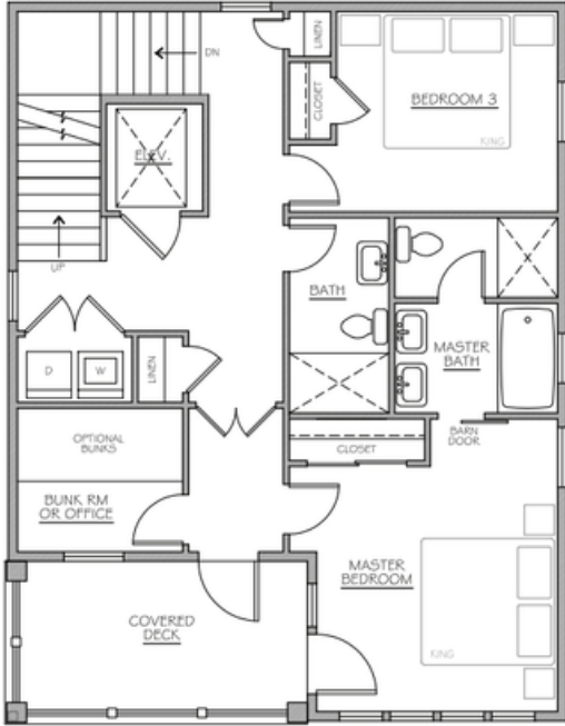
MAIN LEVEL
