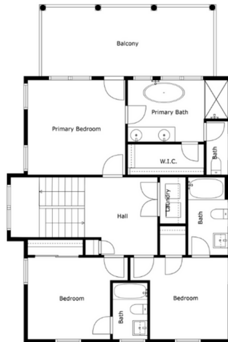
SECOND LEVEL
