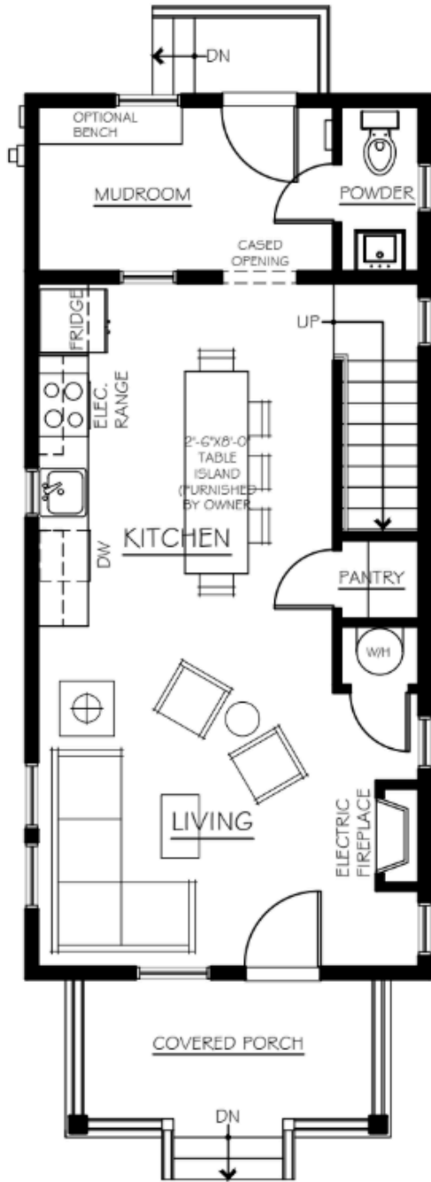
MAIN LEVEL
